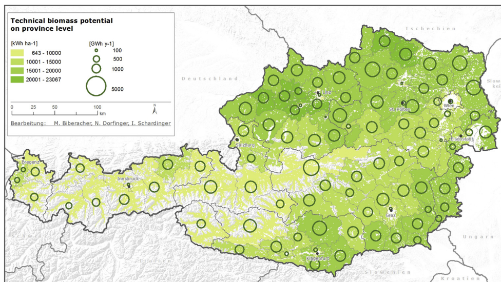
Fig. 6 – Technical biomass energy potential for Austria aggregated to 250 m cells (raster in background) and for districts (with circles at their geographic centres, and circle sizes representing the absolute biomass potential). Translated from ref. [59].
