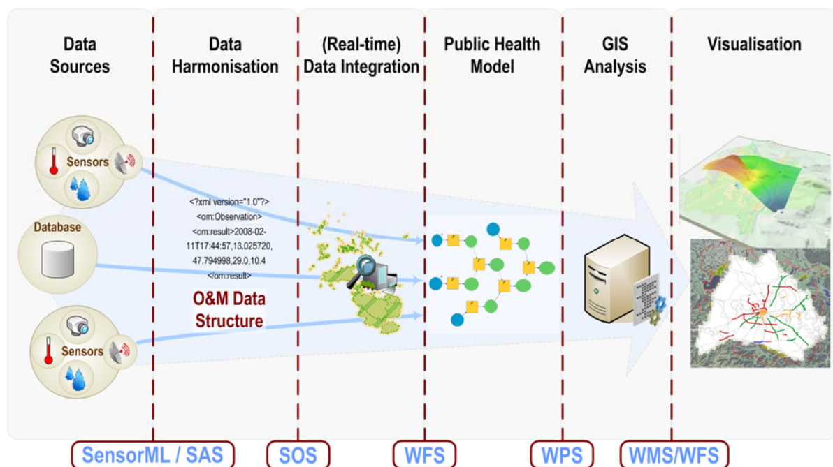
Figure 1 Common Scents – Modular Standardised Infrastructure.
